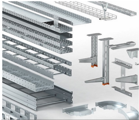
Cable Management System
